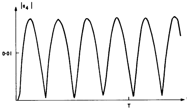
FIG. 4. Amplitude of the m = 4 azimuthal mode versus time, measured at r = 6.0 .
